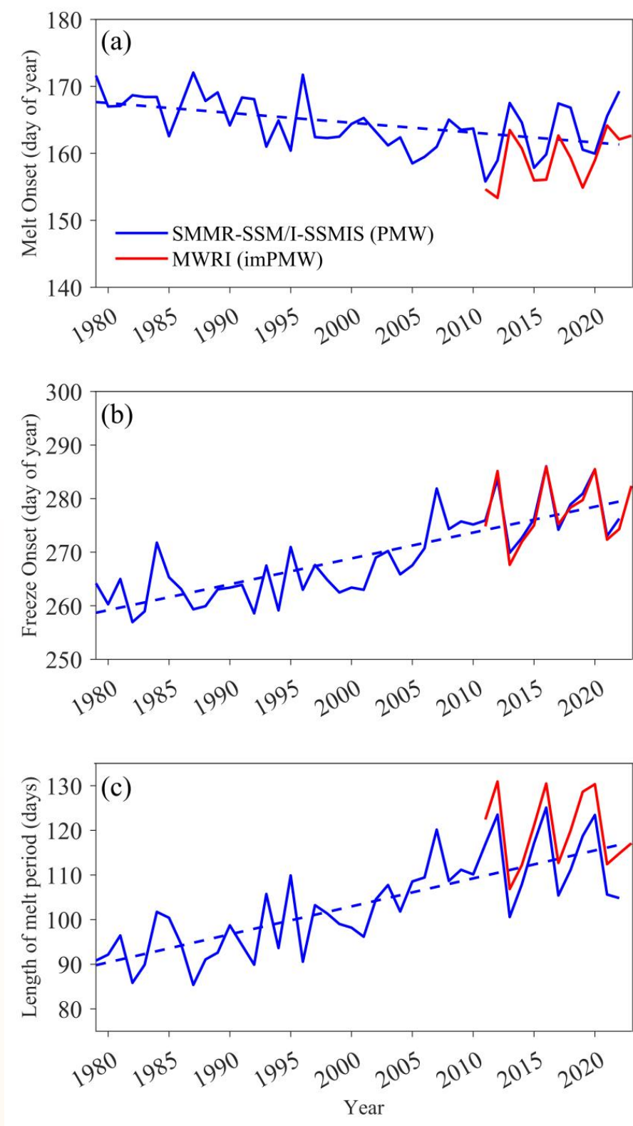
Figure 2.9 Time series of annual averages north of 70°N of (a) the melt onset, (b) the freeze onset, and (c) the length of melt season for data from NASA (blue) and OUC (red)
