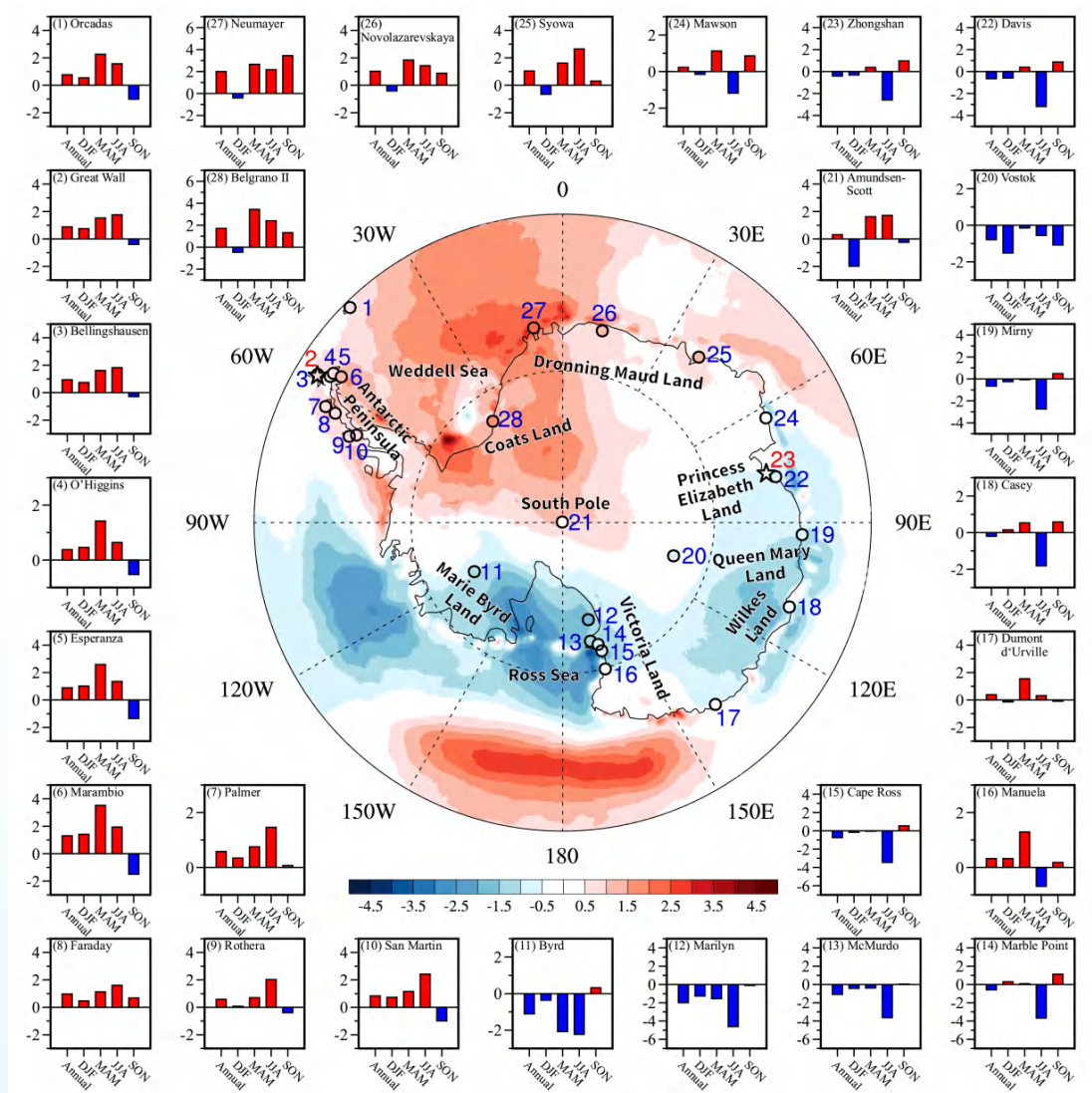
Figure 1.1 Spatial distribution of the 2023 annual mean temperature anomalies in Antarctica and the annual and seasonal mean temperature anomalies at various stations (unit: ^{\circ}\text{C} )
