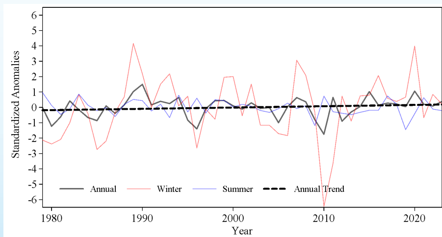
Figure 1.11 Standardized Anomalies of Arctic Oscillation index during 1979–2023
